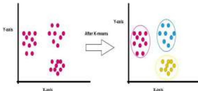
Fig 1. k-means clustering
